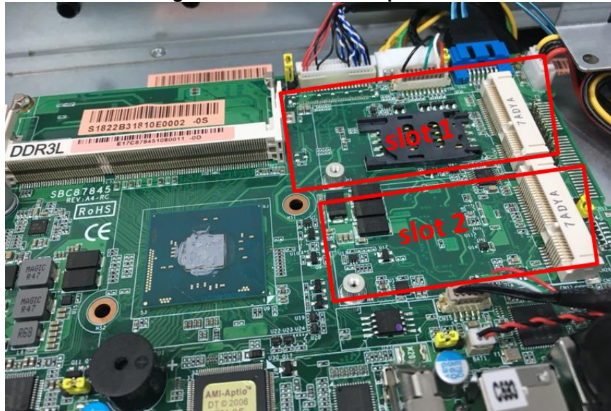
Figure 2-11 Slots 1 and 2 spots
