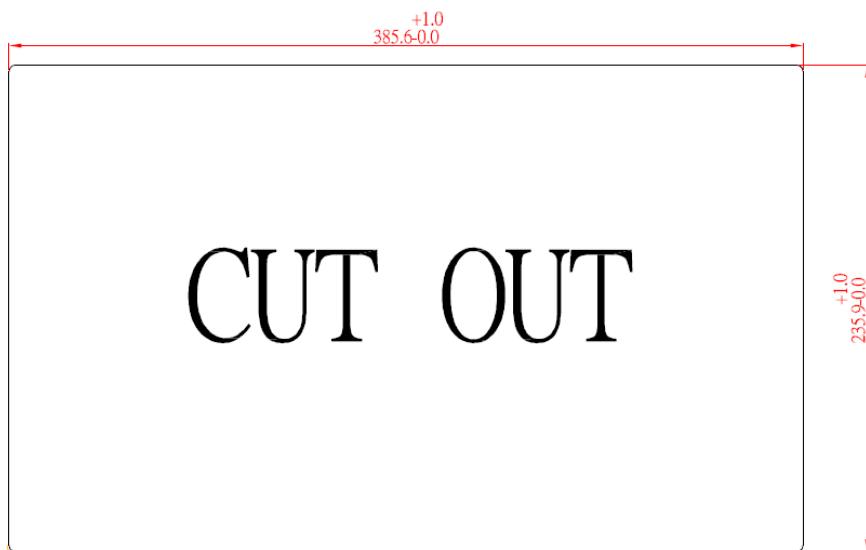
Diagram 1-3 Cutting-out dimensions of the GOT315WL-845-PCT
