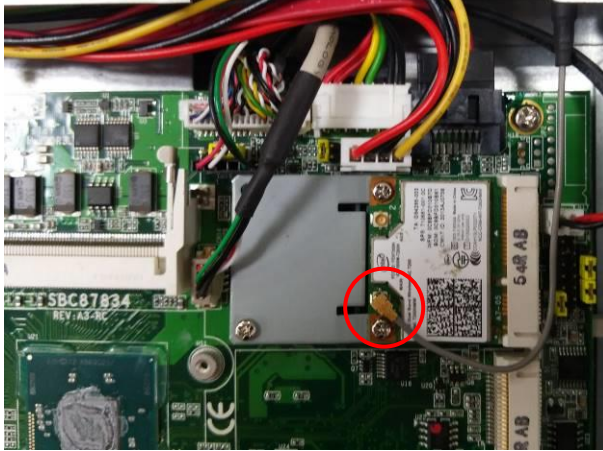
Figure 2-13 Connecting the antenna to the wireless LAN card
