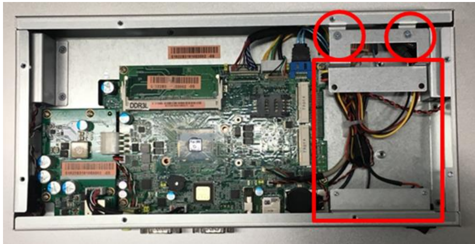
Figure 2-5 Separating the bracket from the HDD tray
