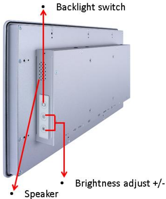
Figure 1-3 Side view of the GOT315WL-845-PCT
