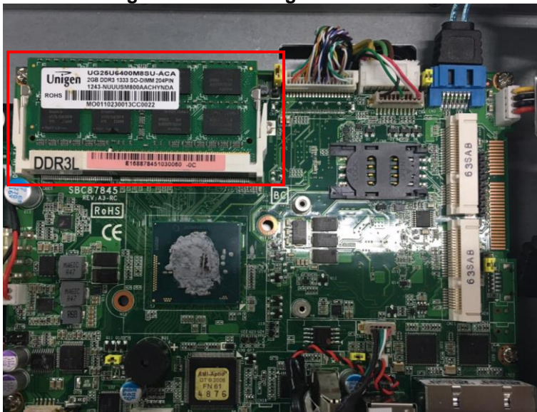
Figure 2-10 Inserting a DRAM into the DIMM
