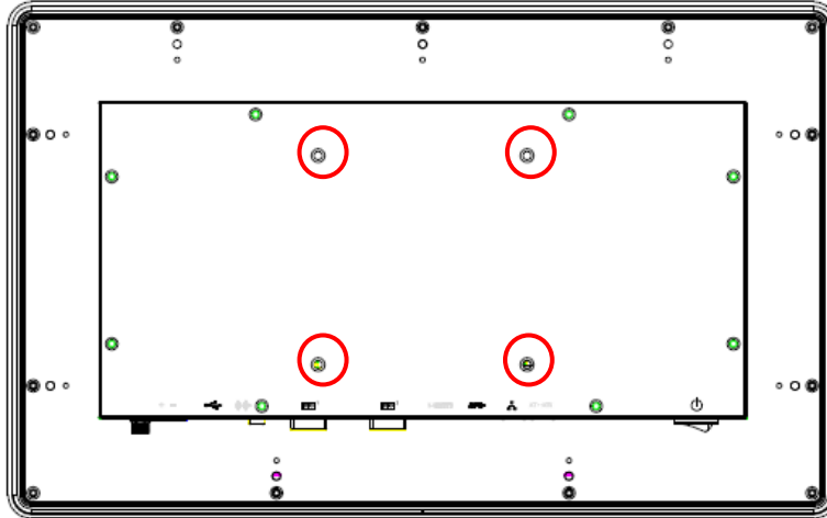
Diagram 2-3 VESA mount (back chassis)
