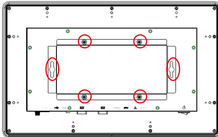
Diagram 2-4 Wall mount (back chassis)
