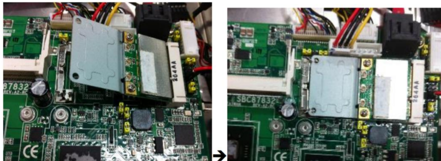
Figure 2-12 Inserting and securing a wireless LAN card
