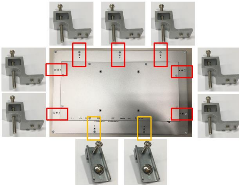
Figure 2-2 Panel mount kit
