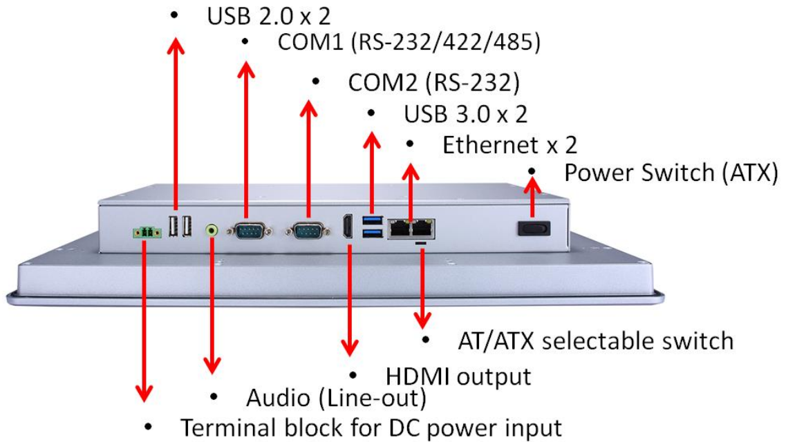
Figure 1-2 Bottom view of the GOT315WL-845-PCT
