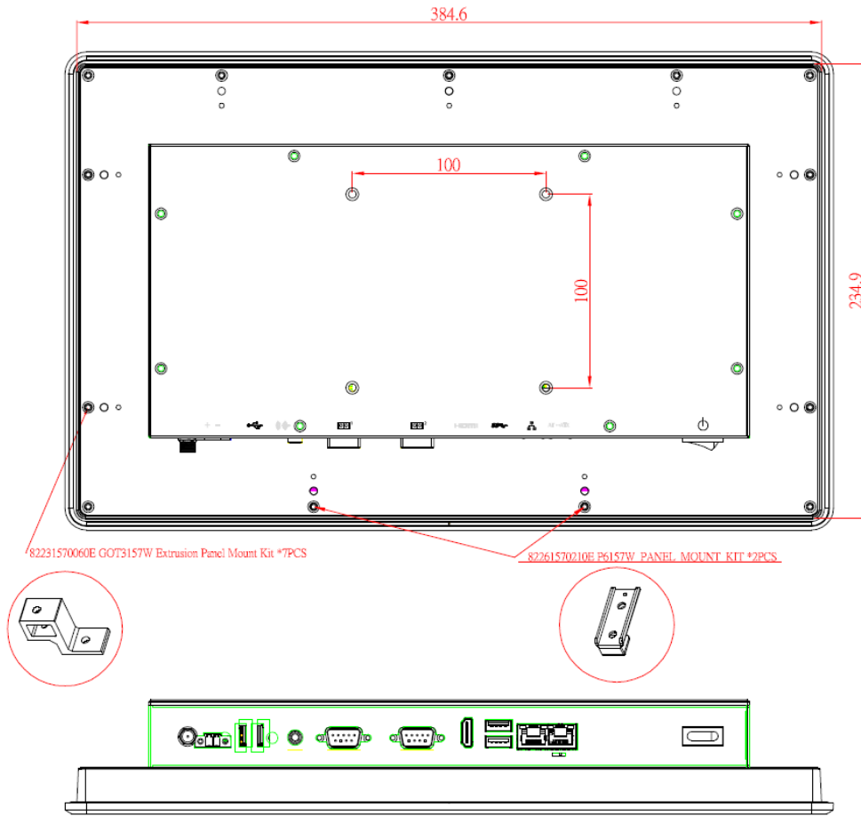
Diagram 1-2 Back outline of the GOT315WL-845-PCT
