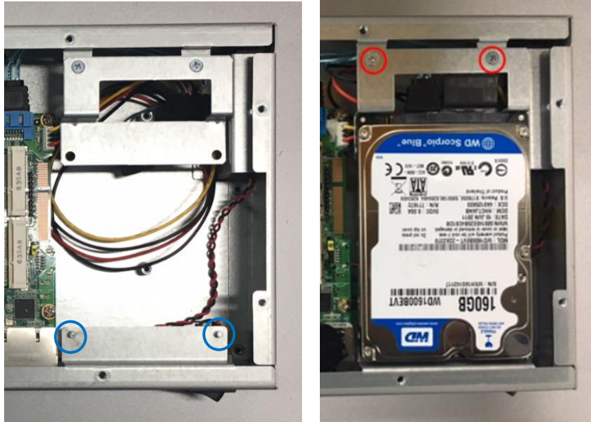
Figure 2-7 Putting the bracket back to the HDD tray
