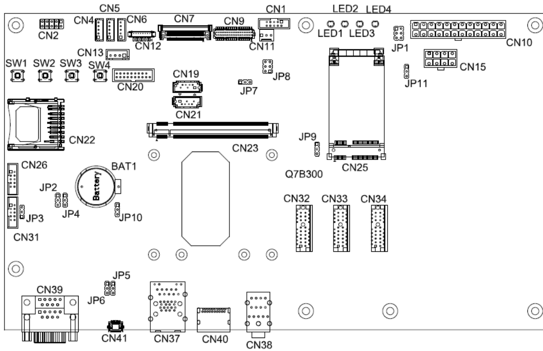
Top View
